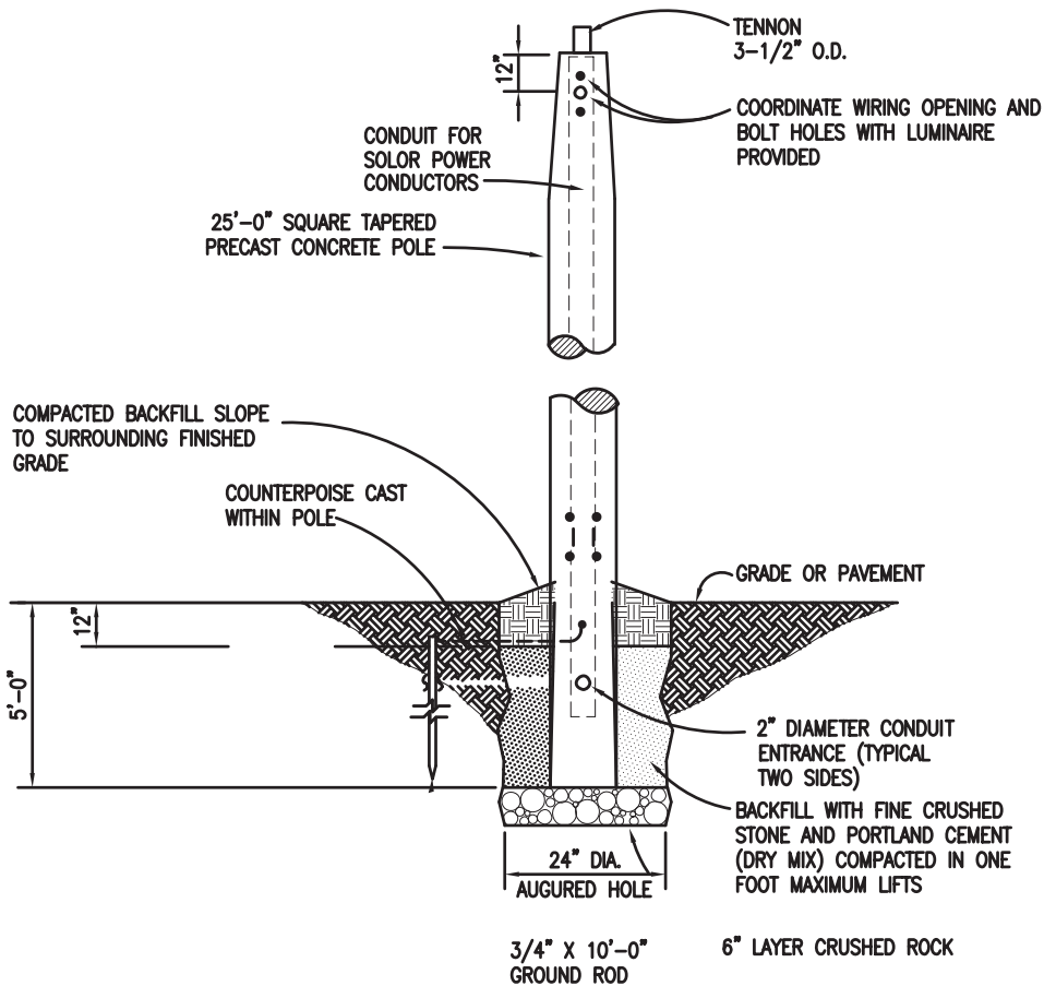
POLE INSTALLATION DETAIL FIXTURE "H" NOT TO SCALE
